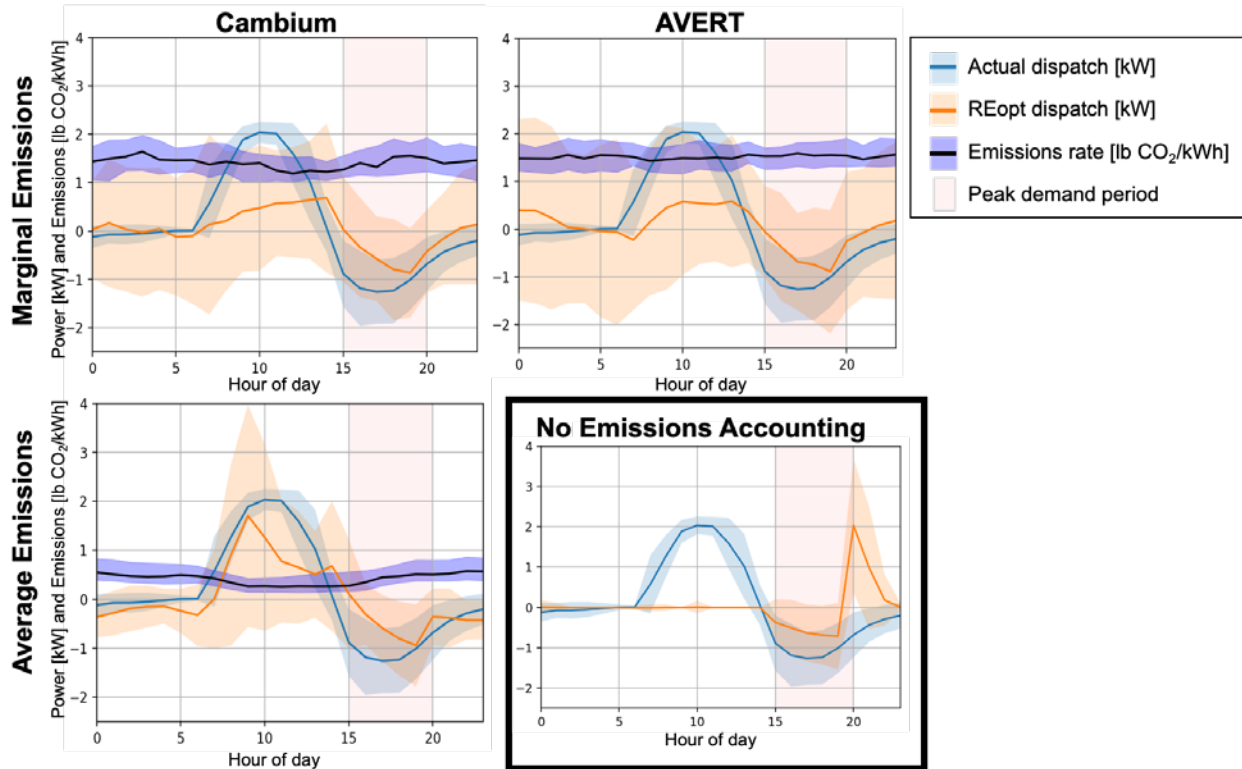
Figure 11. Daily actual battery dispatch (blue) and REopt bill savings- and emissions-optimal dispatch when using varying emissions data sets (orange) for Home A
