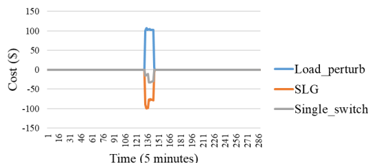
Fig. 11. System generation cost differences between cyber-physical cases and base case
