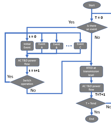
Fig. 7. The simulation flow of cyber-event emulation in the T&D co-simulation
