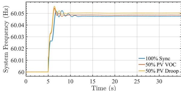
Fig. 3. The weighted system frequency in the IEEE 39-bus test system during a load trip.
