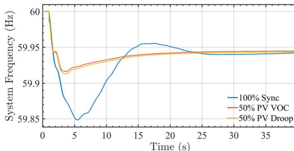
Fig. 7. The weighted system frequency in the microWECC test system during a generation trip.
