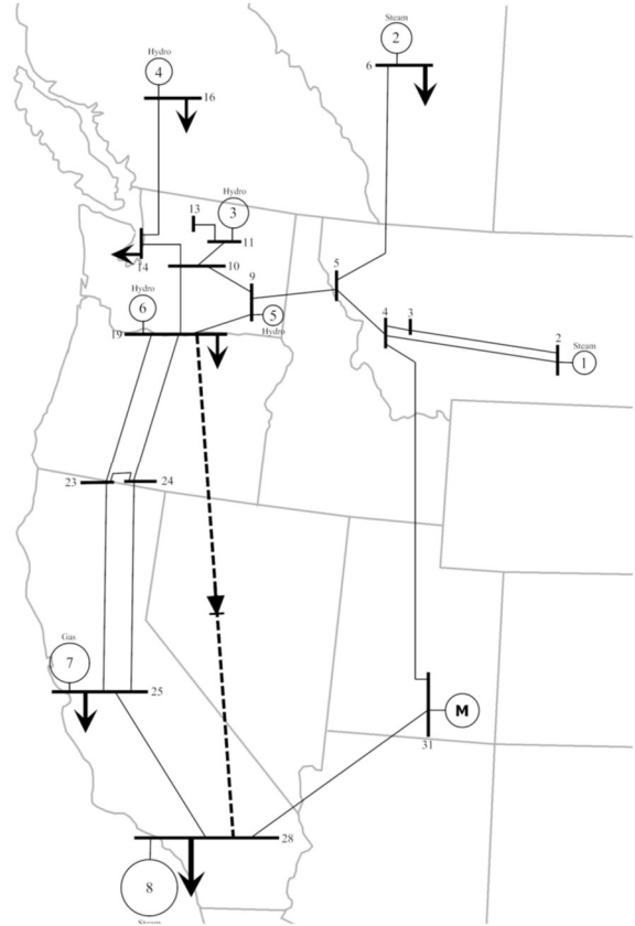
Fig. 2. The microWECC test system [11].
