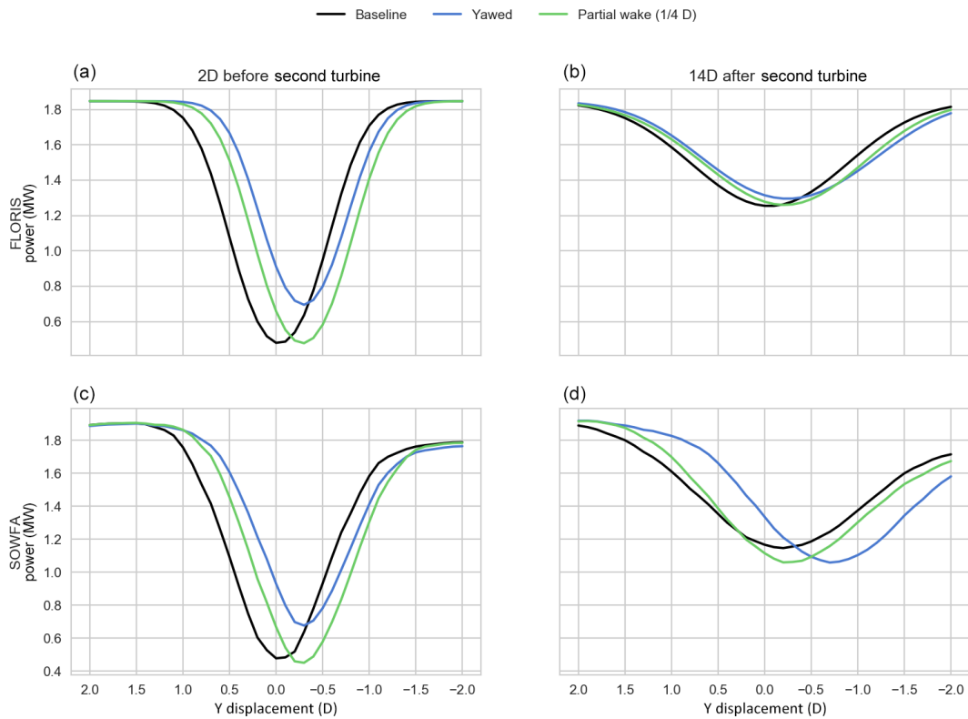
Figure 9. Power of a hypothetical turbine in baseline, yawed (+25°), and partial wake. Panels (a) and (c) shows the power profile 2 diameters (D) before the second turbine, while panels (b) and (d) is 14 D behind.
