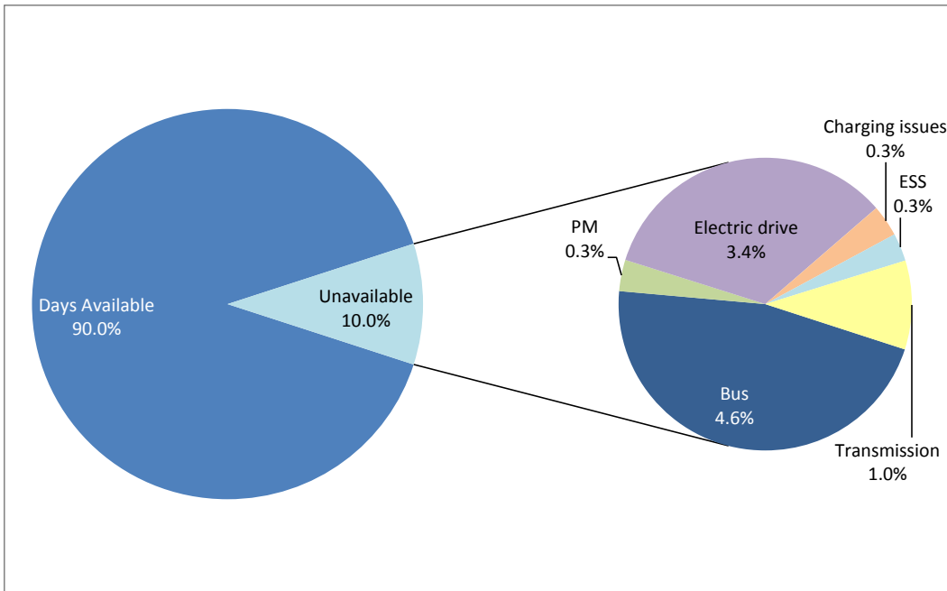
Figure 9. Reasons for unavailability for the Foothill Transit BEBs
