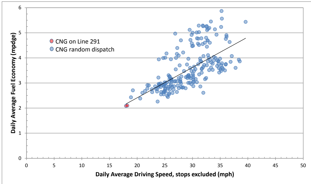
Figure 13. Fuel economy vs. average driving speed for the instrumented CNG buses
