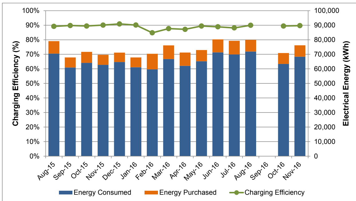
Figure 15. Monthly energy consumption and overall charging efficiency for the BEBs
