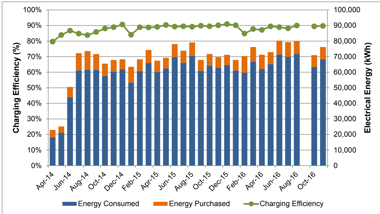
Figure D-5. Monthly energy consumption and overall charging efficiency for the BEBs
