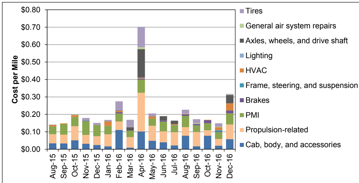
Figure 19. Monthly maintenance cost per mile by vehicle system for the CNG buses
