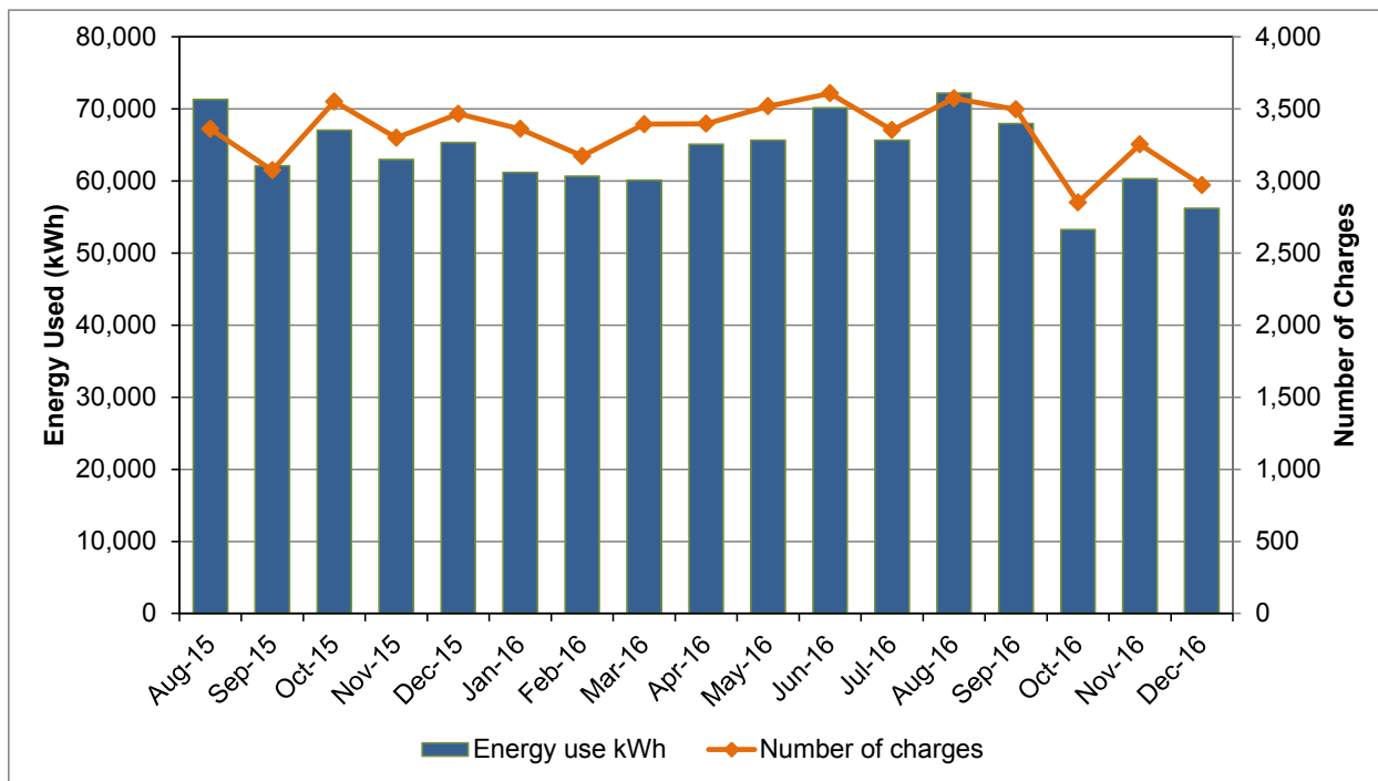
Figure 11. Monthly energy use and number of charges for the BEB fleet
