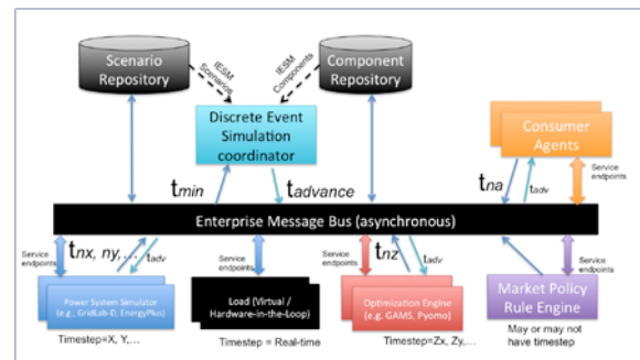
Figure 1. Integrated Energy System Model (IESM) architecture
