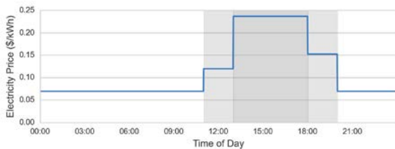
Figure 3. Time-of-use pricing profile for weekdays. All weekend hours are off-peak and have the lowest price
