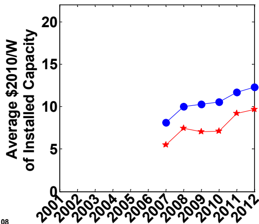
Capacity < 500 kW
