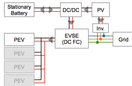
Figure 4: Renewable fast charging station schematic
