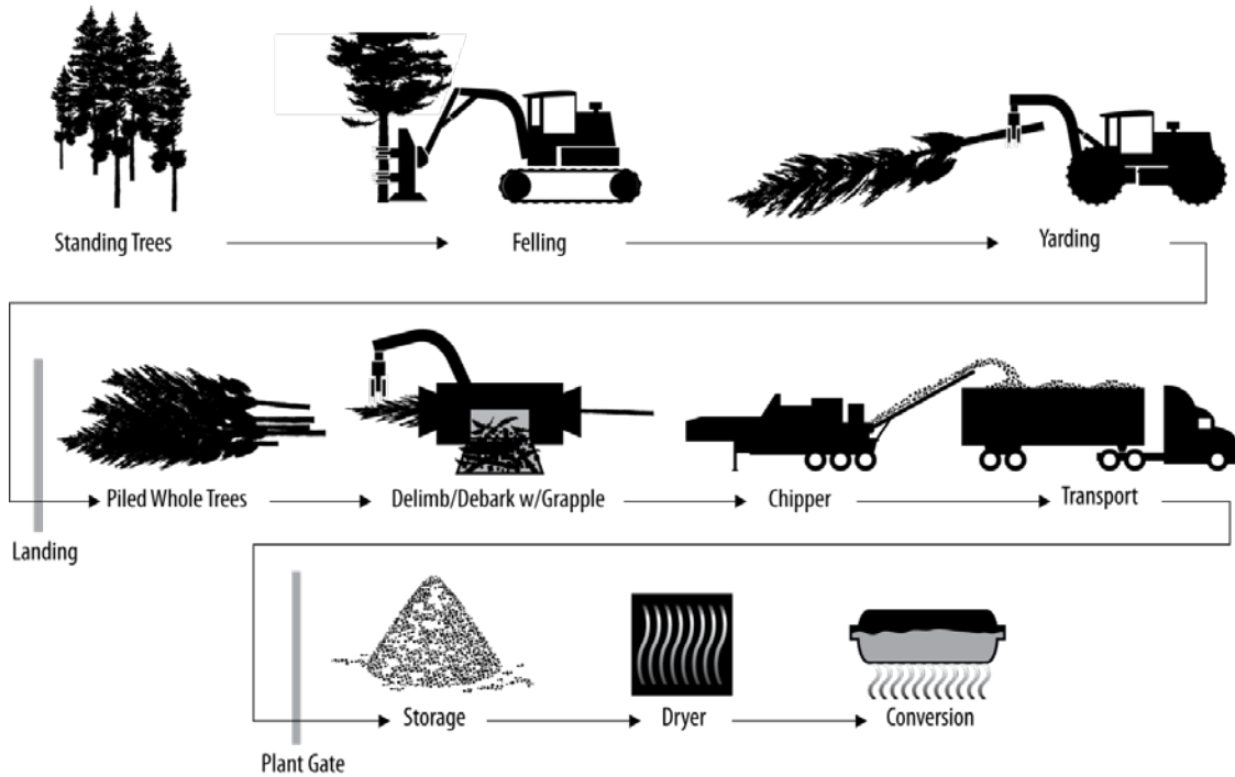
Figure 5. Woody biomass feedstock supply system
