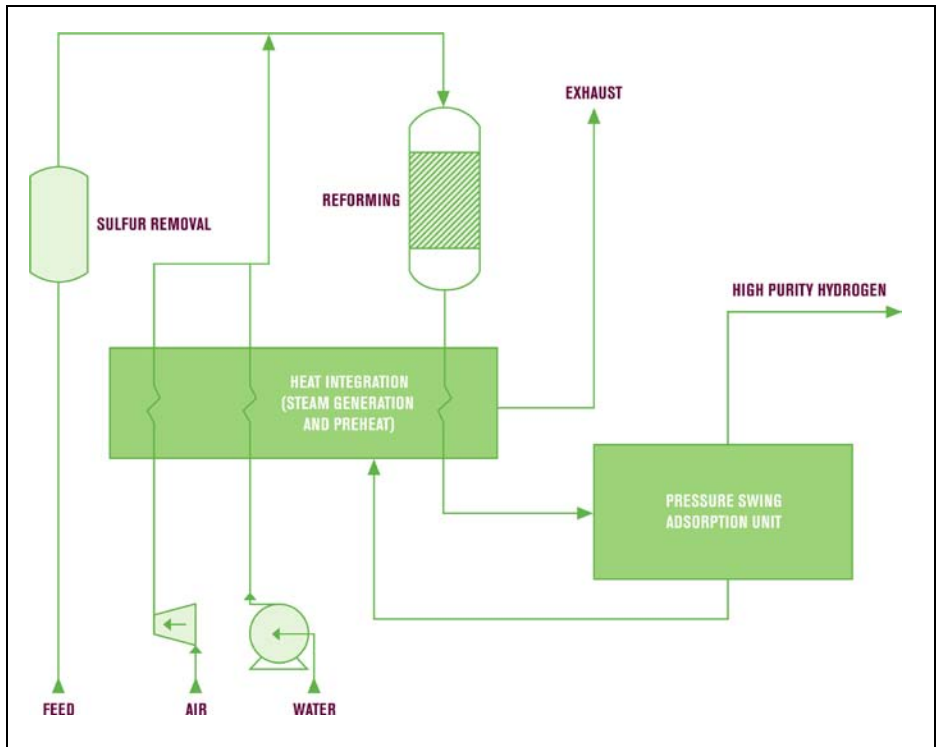
Figure D-5. HyRadix hydrogen production process (Courtesy of HyRadix)
