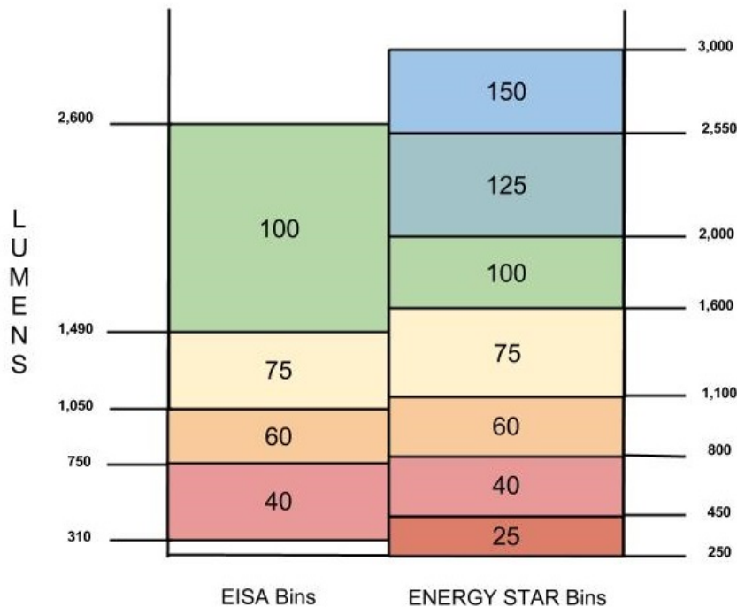
Figure 2. Baseline wattage by lumens, EISA versus ENERGY STAR 12
