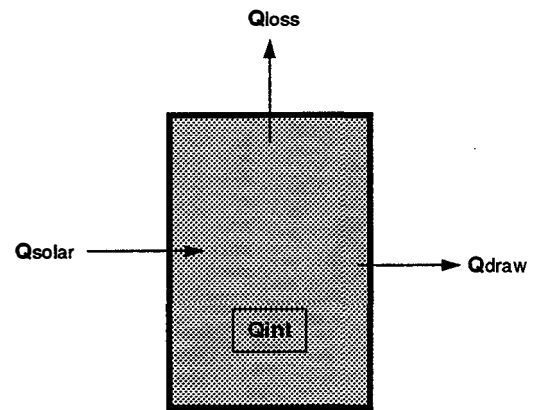
Fig. 2 Tank energy balance, showing energy gains and losses for the solar storage. In one-tank systems, the control volume is drawn below the auxiliary storage.
