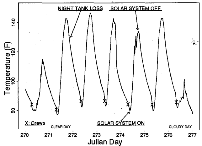
Fig. 6 Tank temperature versus time at site 2. The probe was located near the middle of solar storage, identically to site 1. Compare the rapid nighttime decrease in decrease of site 2 versus that of site 1.
