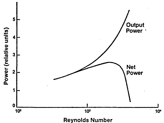
Fig. 4 - TEG power output and heat exchanger-TEG system power output
