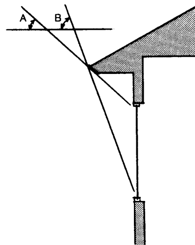
South Overhang Sizing In Rock Springs, an ideally sized south overhang should allow full exposure of the window when the sun has a noon altitude of 29 degrees (angle A) and fully shade the window when the sun has a noon altitude of 66 degrees (angle B).
