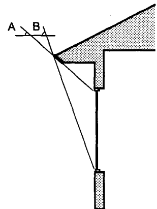
South Overhang Sizing In Green Bay, an ideally sized south overhang should allow full exposure of the window when the sun has a noon altitude of 27 degrees (angle A) and fully shade the window when the sun has a noon altitude of 64 degrees (angle B).
