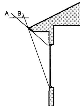
South Overhang Sizing In Spokane, an ideally sized south overhang should allow full exposure of the window when the sun has a noon altitude of 23 degrees (angle A) and fully shade the window when the sun has a noon altitude of 60 degrees (angle B).
