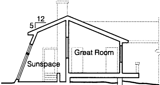
ABOVE GRADE SECTION
