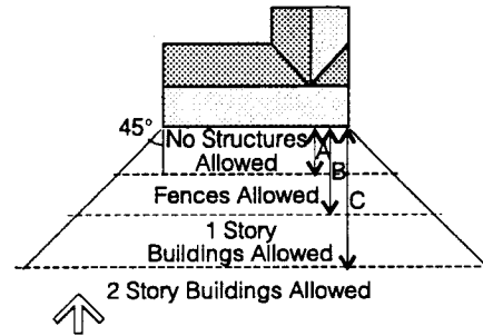
Ideal Solar Access Buildings, trees or other obstructions should not be located so as to shade the south wall of solar buildings. At this latitude, A = 27 ft., B = 47 ft., and C = 109 ft.
