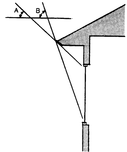
South Overhang Sizing In Whidbey Island, an ideally sized south overhang should allow full exposure of the window when the sun has a noon altitude of 23 degrees (angle A) and fully shade the window when the sun has a noon altitude of 60 degrees (angle B).
