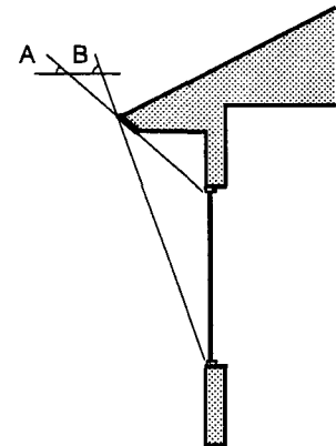
South Overhang Sizing In Salt Lake City, an ideally sized south overhang should allow full exposure of the window when the sun has a noon altitude of 30 degrees (angle A) and fully shade the window when the sun has a noon altitude of 67 degrees (angle B).
