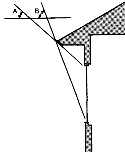
South Overhang Sizing In San Antonio, an ideally sized south overhang should allow full exposure of the window when the sun has a noon altitude of 41 degrees (angle A) and fully shade the window when the sun has a noon altitude of 78 degrees (angle B).
