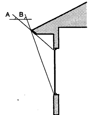
South Overhang Sizing In Austin, an ideally sized south overhang should allow full exposure of the window when the sun has a noon altitude of 41 degrees (angle A) and fully shade the window when the sun has a noon altitude of 78 degrees (angle B).
