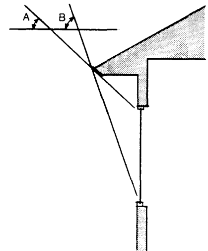
South Overhang Sizing In Charleston, an ideally sized south overhang should allow full exposure of the window when the sun has a noon altitude of 38 degrees (angle A) and fully shade the window when the sun has a noon altitude of 75 degrees (angle B).
