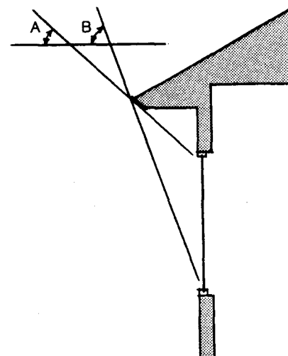
South Overhang Sizing In Long Island, an ideally sized south overhang should allow full exposure of the window when the sun has a noon altitude of 30 degrees (angle A) and fully shade the window when the sun has a noon altitude of 67 degrees (angle B).
