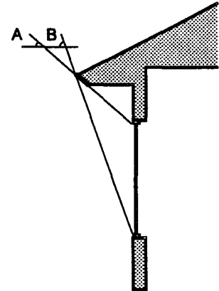
South Overhang Sizing In Cherry Point, an ideally sized south overhang should allow full exposure of the window when the sun has a noon altitude of 36 degrees (angle A) and fully shade the window when the sun has a noon altitude of 73 degrees (angle B).
