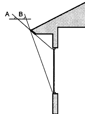
South Overhang Sizing In Boston, an ideally sized south overhang should allow full exposure of the window when the sun has a noon altitude of 29 degrees (angle A) and fully shade the window when the sun has a noon altitude of 66 degrees (angle B).
