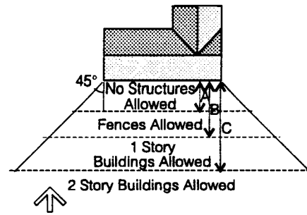
Ideal Solar Access Buildings, trees or other obstructions should not be located so as to shade the south wall of solar buildings. At this latitude, A = 15 ft., B = 27 ft., and C = 61 ft.
