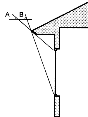
South Overhang Sizing In Chicago, an ideally sized south overhang should allow full exposure of the window when the sun has a noon altitude of 29 degrees (angle A) and fully shade the window when the sun has a noon altitude of 66 degrees (angle B).
