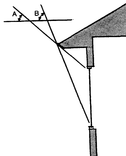
South Overhang Sizing In Denver, an ideally sized south overhang should allow full exposure of the window when the sun has a noon altitude of 31 degrees (angle A) and fully shade the window when the sun has a noon altitude of 68 degrees (angle B).
