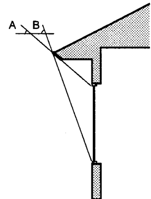
South Overhang Sizing In Colorado Springs, an ideally sized south overhang should allow full exposure of the window when the sun has a noon altitude of 32 degrees (angle A) and fully shade the window when the sun has a noon altitude of 69 degrees (angle B).
