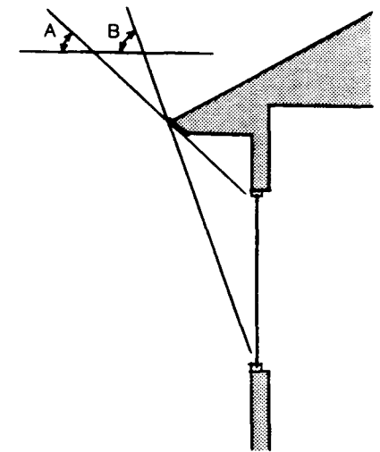
South Overhang Sizing In San Jose, an ideally sized south overhang should allow full exposure of the window when the sun has a noon altitude of 33 degrees (angle A) and fully shade the window when the sun has a noon altitude of 70 degrees (angle B).
