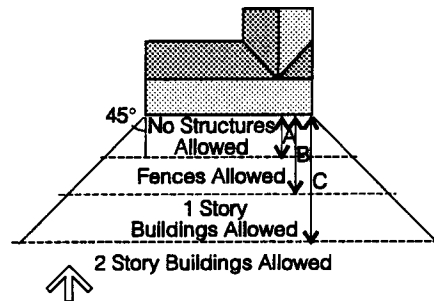
Ideal Solar Access Buildings, trees or other obstructions should not be located so as to shade the south wall of solar buildings. At this latitude, A = 8 ft., B = 15 ft., and C = 34 ft.
