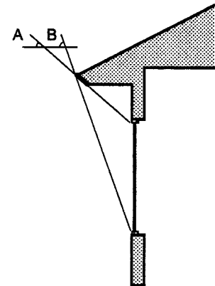
South Overhang Sizing In Tucson, an ideally sized south overhang should allow full exposure of the window when the sun has a noon altitude of 39 degrees (angle A) and fully shade the window when the sun has a noon altitude of 76 degrees (angle B).
