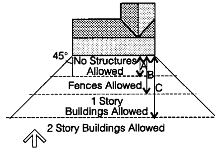
Ideal Solar Access Buildings, trees or other obstructions should not be located so as to shade the south wall of solar buildings. At this latitude, A = 10 ft., B = 17 ft., and C = 38 ft.
