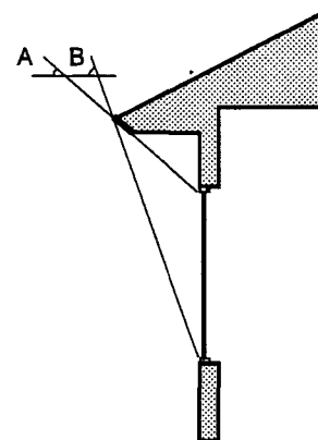
South Overhang Sizing In Prescott, an ideally sized south overhang should allow full exposure of the window when the sun has a noon altitude of 36 degrees (angle A) and fully shade the window when the sun has a noon altitude of 73 degrees (angle B).
