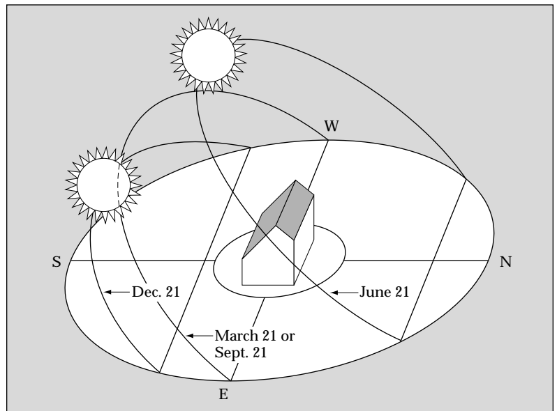
In northern latitudes, the sun is much lower in the sky in the winter than in the summer. For this reason, vertical glazing receives much more solar gain in the coldest part of the year. Sloped glazing takes in the most solar radiation in the summer.
