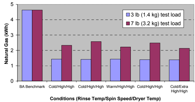
Figure 7. Clothes-dryer natural gas use under various operating conditions
