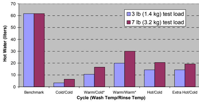
Figure 4. Clothes washer hot water use under various operating conditions. Extra rinse used for Warm/Cold and 3 lb (1.4 kg) Warm/Warm cycles.
