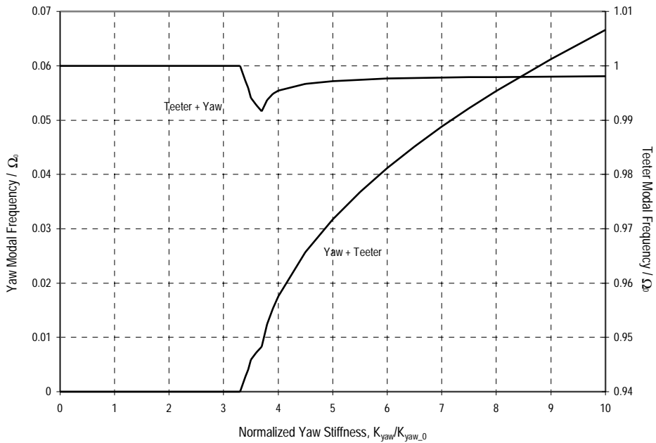
Fig. 6a. Effect of yaw stiffness on modal frequencies (nominal stiffness, K_0 = 570 \text{ Nm/rad} )
