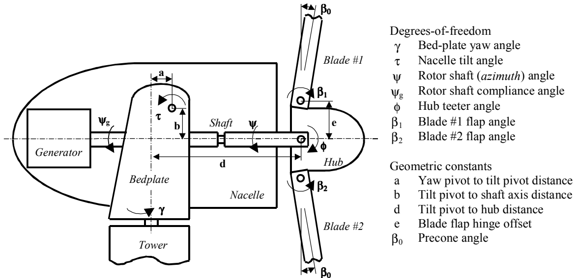
Fig. 1. Wind turbine schematic showing degrees of freedom and geometric parameters.
