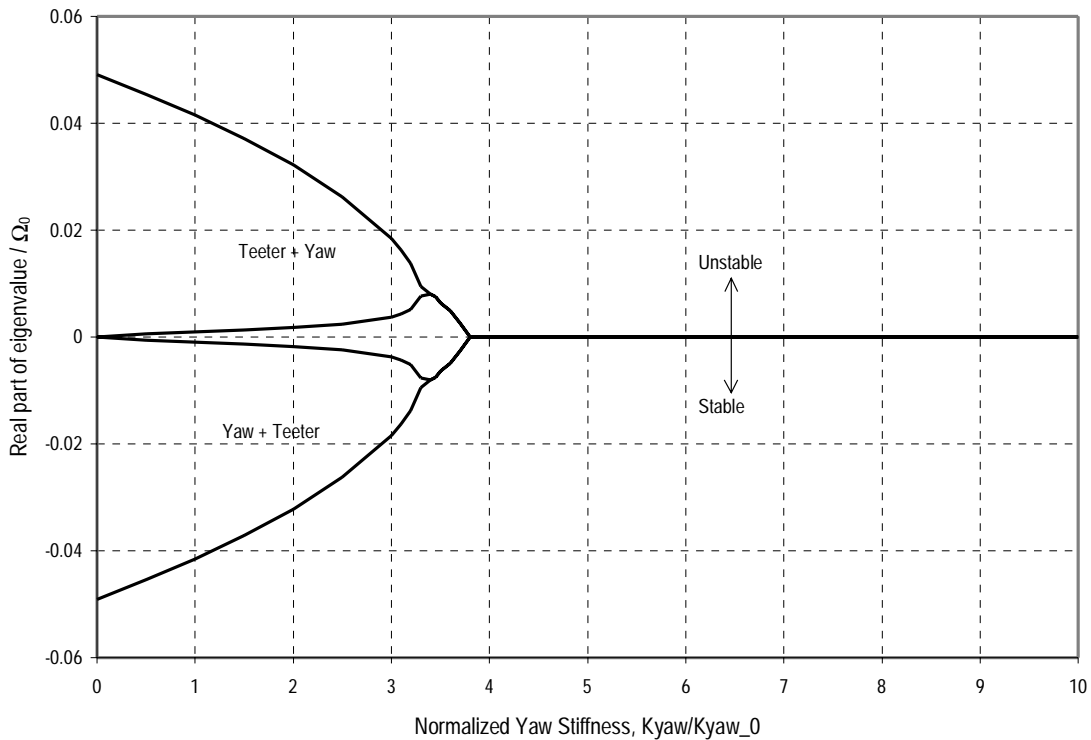
Fig. 6b. Effect of yaw stiffness on modal damping (nominal stiffness, K_0 = 570 \text{ Nm/rad} )
