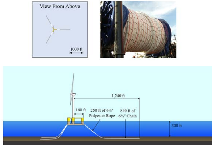
Figure 10. For the hybrid mooring design, the overview graphic (top left) shows mooring lines from above, example synthetic fiber rope (top right), and the footprint of the platform and mooring lines (bottom middle). Top left and bottom middle graphics created by Stein Housner and Matt Hall, NREL; top right photo from Lankhorst Offshore
