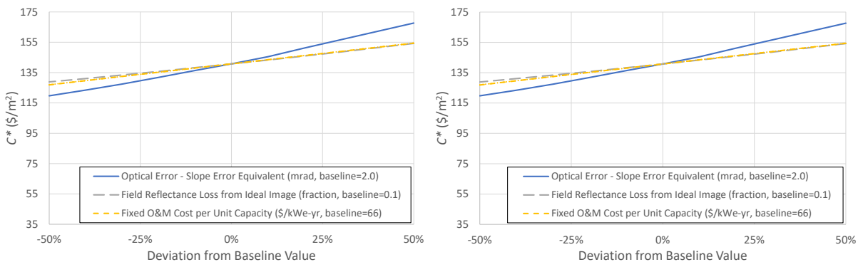
Figure 3. LCOH parametric analysis on impact to equivalent breakeven installed heliostat cost, C*, for a large-scale electric plant case study, using baseline installed capital costs of $50/m 2 and $140/m 2 on the left and right plots, respectively. Baseline values of 1.29 and 2.05 cents/kWh are located on the centerline of the horizontal axis for each case.
