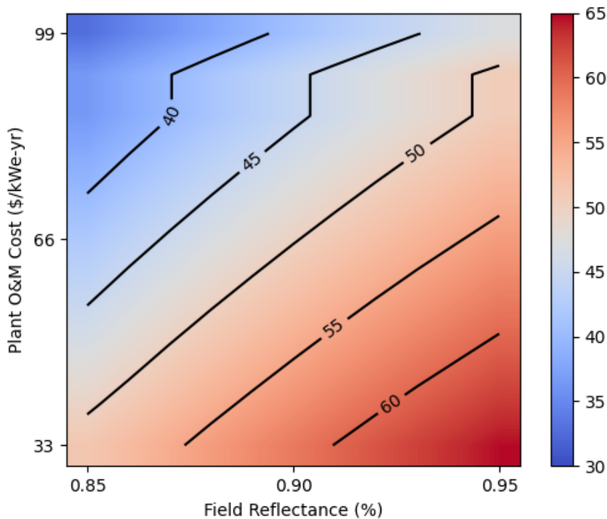
Figure 4. Heat map depicting equivalent breakeven installed cost as reflectance and O&M costs vary. Contour lines indicate capital cost levels. Baseline cost of \$50/\text{m}^2 is located at the center of the graph.
