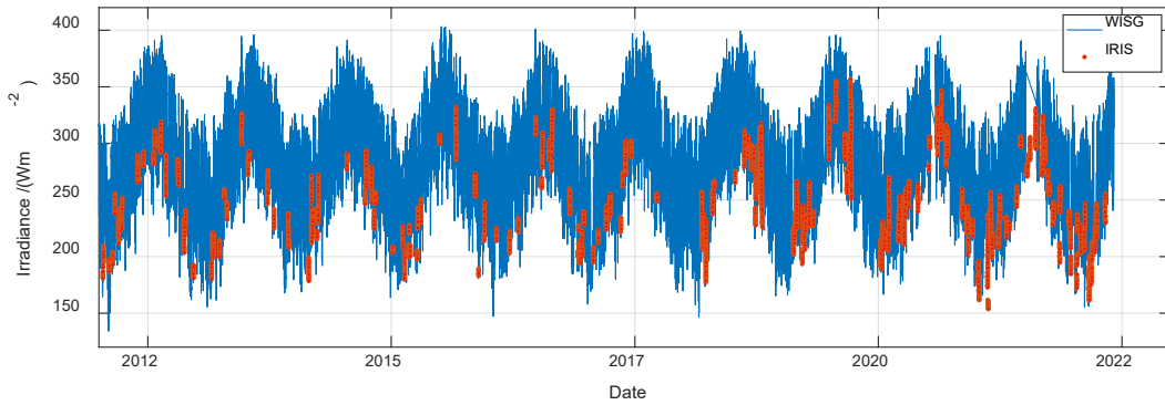
FIGURE 1 Atmospheric longwave irradiance measurements at PMOD/WRC from the WISG (blue), and during cloud-free nights with the IRIS radiometers (red).
