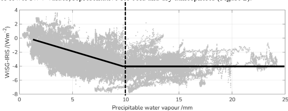
FIGURE 2 Difference between WISG and IRIS with respect to Integrated Water Vapor (IWV) for the simultaneous measurements shown in Figure 1.
