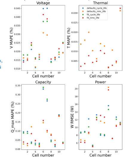
Component model accuracy for 11 cells under different conditions. Accuracy is lowest at non-room temperature conditions.
