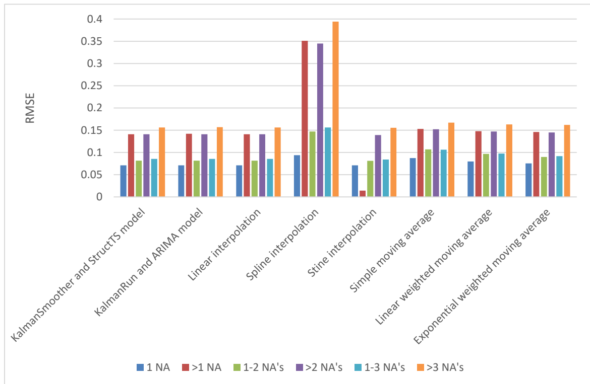
Fig. 3: Resulting RMSE values by imputation method across six NA bin sizes for Bondville, IL NSRDB data
