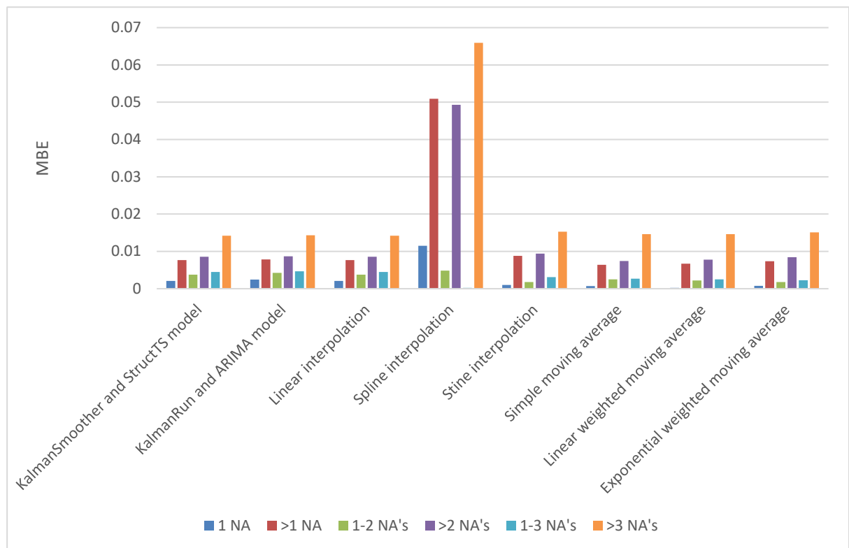
Fig. 5: Resulting absolute MBE values by imputation method across six NA bin sizes for Bondville, IL NSRDB data
