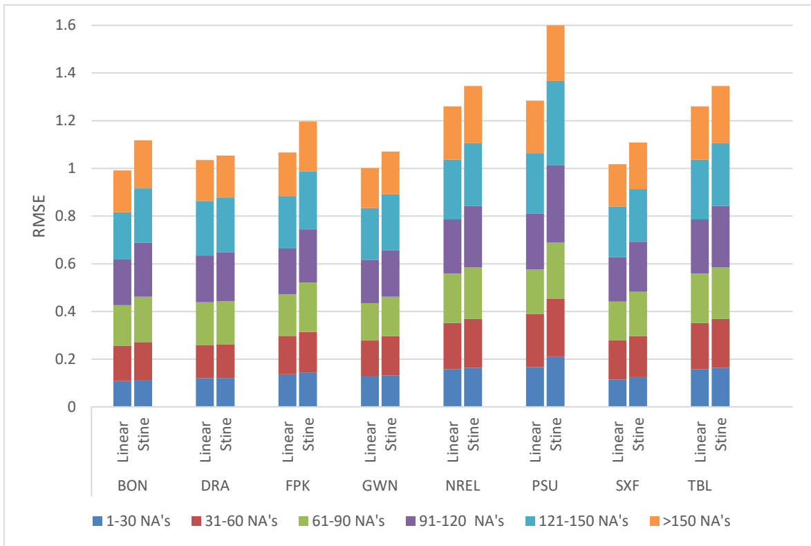
Fig. 6: Resulting RMSE by location and interpolation method for ground measurement data
