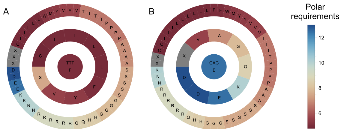
Figure 1. Codon accessibility examples. The center circle denotes the wild-type codon. The inner ring displays the accessible amino acids via a single-base substitution, and the outer ring represents the two- and three-base change accessibility. Colors correlate with amino acid polar requirements. A. A single-base change within the TTT codon does restrict accessibility to amino acids with low polar requirements and thus does not explore the complete possible amino acid repertoire. Removing the inner ring codons and focusing on codon distance larger than 1 results in a much more balanced library with amino acids spanning across the complete polar requirements spectrum. B. The GAG codon represents a more evolvable codon, representing a variety of amino acids in both rings.
