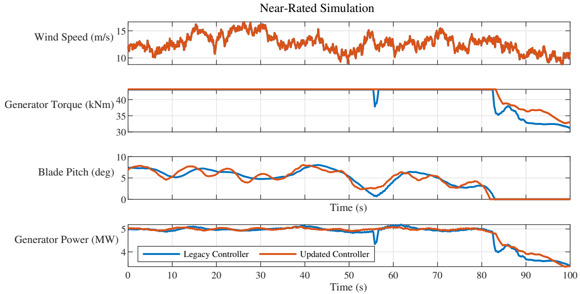
Figure 6. Near-rated simulation results of the NREL 5-MW land-based wind turbine in an incident wind field with an average wind speed of 12 m/s and IEC normal turbulence.
