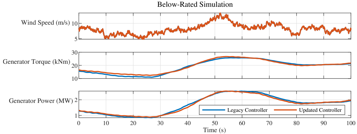
Figure 5. Below-rated simulation results of the NREL 5-MW land-based wind turbine in an incident wind field with an average wind speed of 8 m/s and International Electrotechnical Commission (IEC) normal turbulence.
