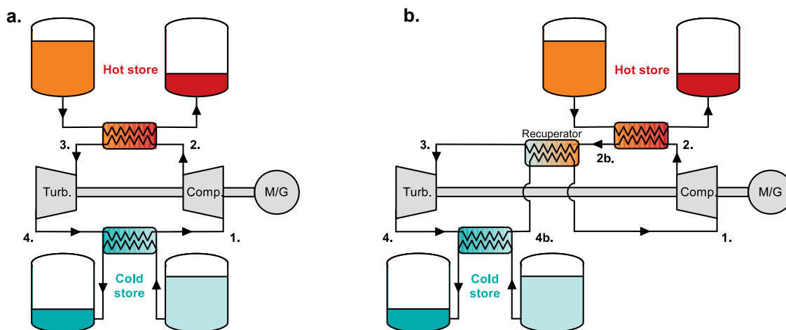
FIGURE 1: Schematic layout of PTES designs during charge. a) The concept used for sCO 2 cycles b) A recuperated cycle with an ideal gas as the working fluid. Key: M/G – motor-generator; Turb. – turbine; Comp. – compressor.
