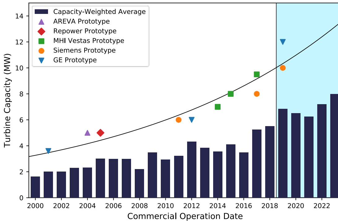
Figure 23. Average commercial offshore wind turbine rating compared to prototype deployment by year
