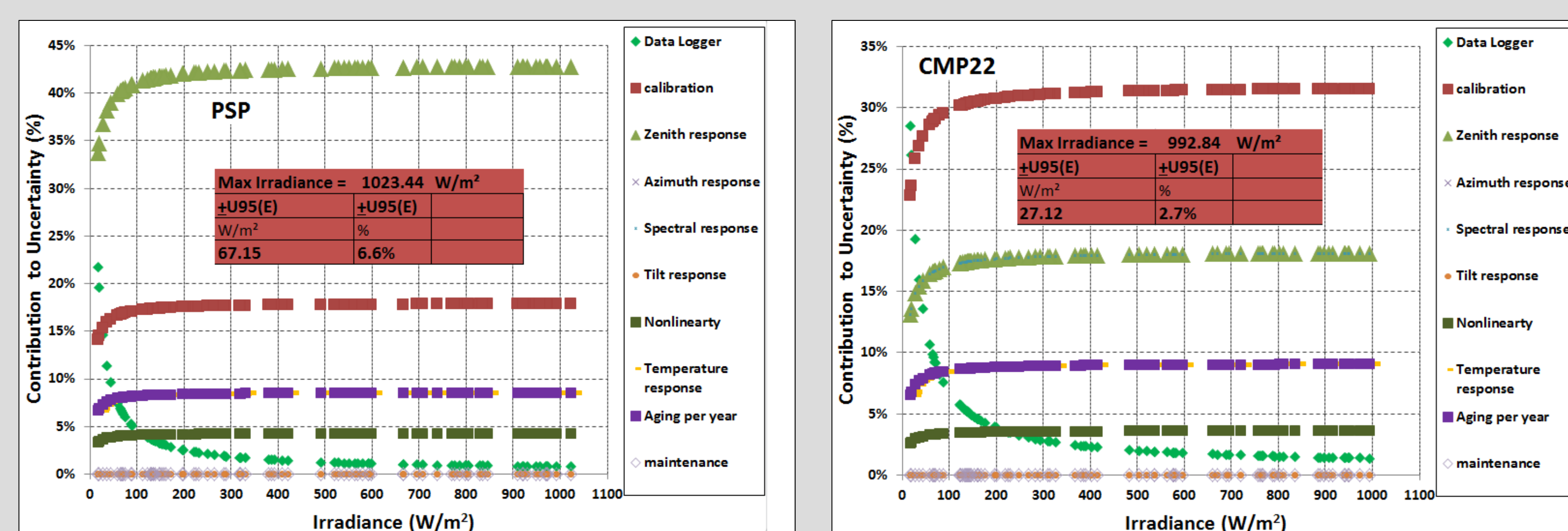
Figure 6. Contribution of sources of uncertainties to the overall uncertainty estimation of pyranometers. Left: PSP; right: CMP22
