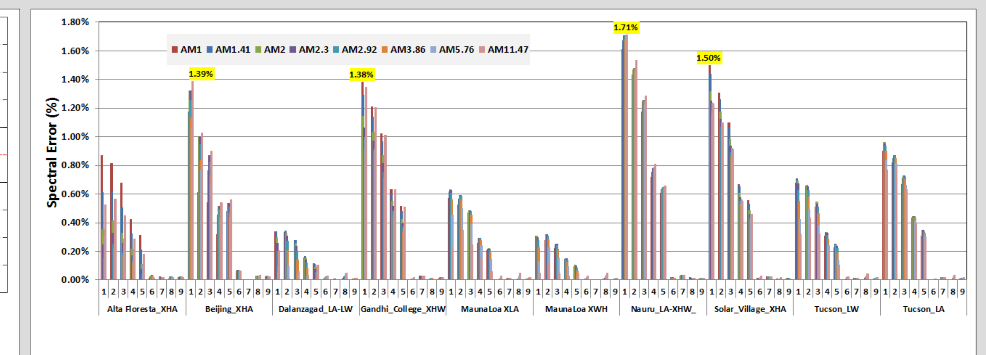
Figure 4. Results showing the spectral error of shortwave radiometers under different air masses (AM) and locations [5]. Note: Spectral irradiance simulation was performed using SMARTS model.
