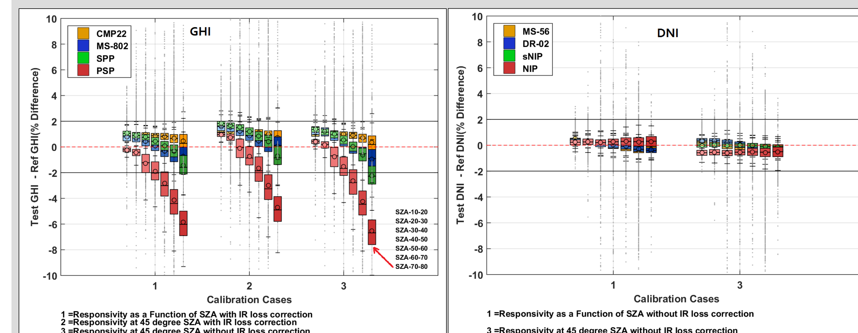
Figure 2. Comparison of NREL's calibration responsivity for clearness index ( K_n ) above 0.6. Differences are shown in percentage and W/m^2 . Left: GHI; right: direct normal irradiance (DNI)
