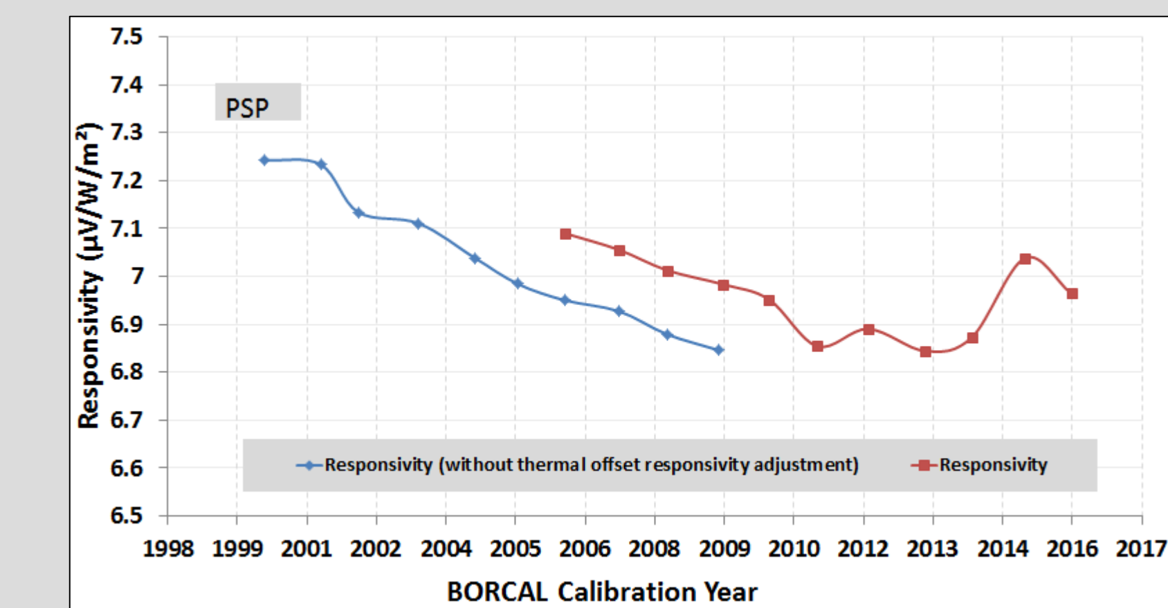
Figure 3. History of instrument at zenith angle = 45^\circ
