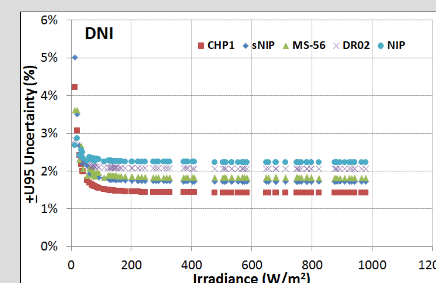
Figure 5. Overall uncertainty for DNI radiometers
