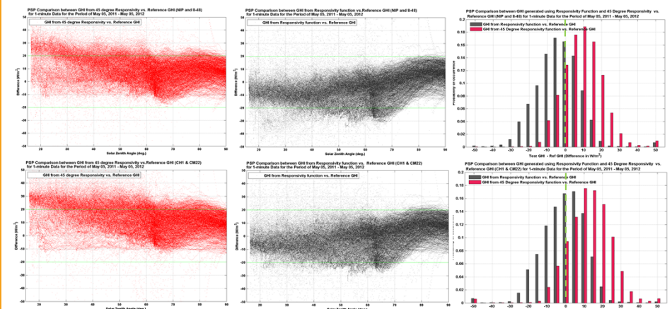
Figure 2. Top figures are Eppley PSP comparison relative to the reference GHI calculated using Eppley NIP (DNI) and 8-48 (DHI) and bottom figures are the same comparison, but the reference is calculated using Kipp and Zonen CH1 (DNI) and CM22 (DHI).
