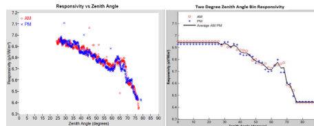
Figure 1. Left figure shows AM and PM responsivity and solar-zenith angle as measured on May 5, 2011. Right figure shows measured responsivity, grouped into AM and PM 2-degree solar-zenith angle bins. These bins were averaged and linearly interpolated to produce a responsivity function by which any discrete responsivity can be calculated.
