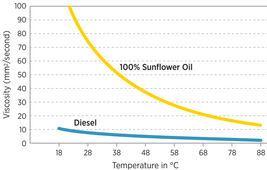
Figure 2. Viscosities of sunflower oil and conventional diesel fuel as a function of temperature.
