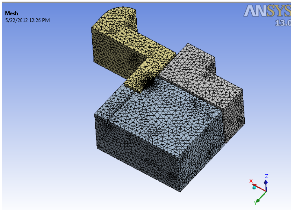
Figure 2. CFD model mesh of the bedroom (light blue), bathroom (gray), and hallway (tan)
