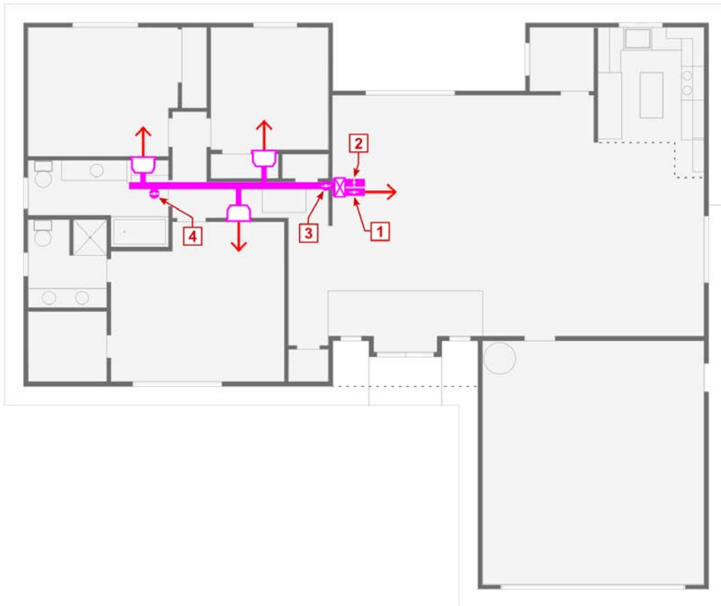
Figure 7. Distribution strategy 2
