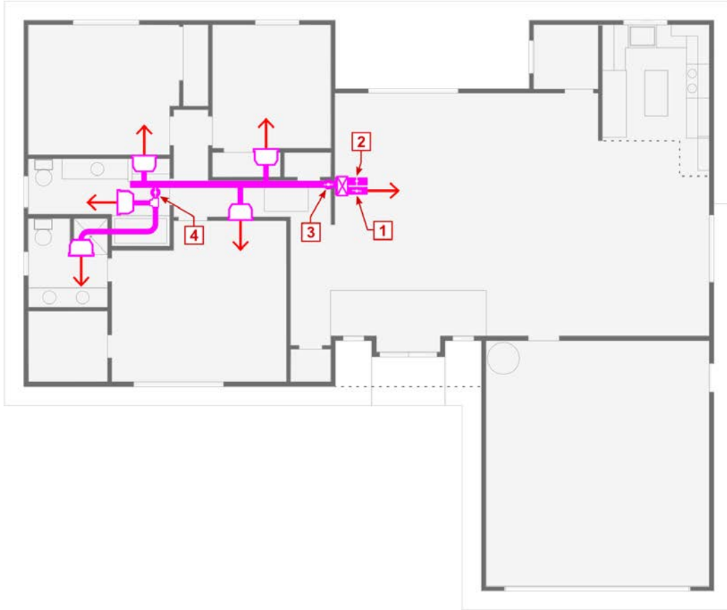
Figure 6. Distribution strategy 1
