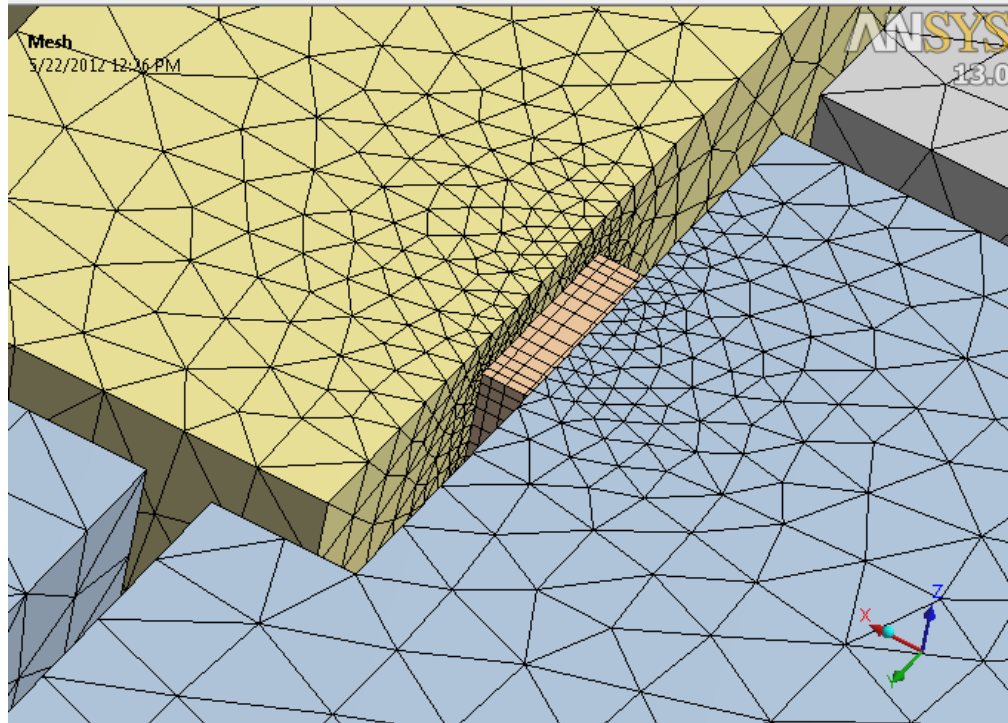
Figure 3. Close-up of CFD model mesh showing the upper transfer grille (pink) connecting the bedroom (light blue) and hallway (tan)
