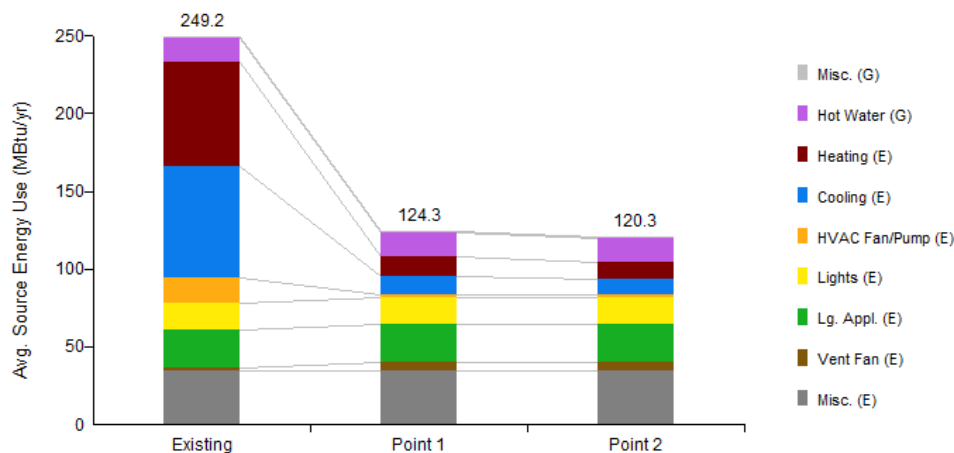
Figure 1. BEopt results
