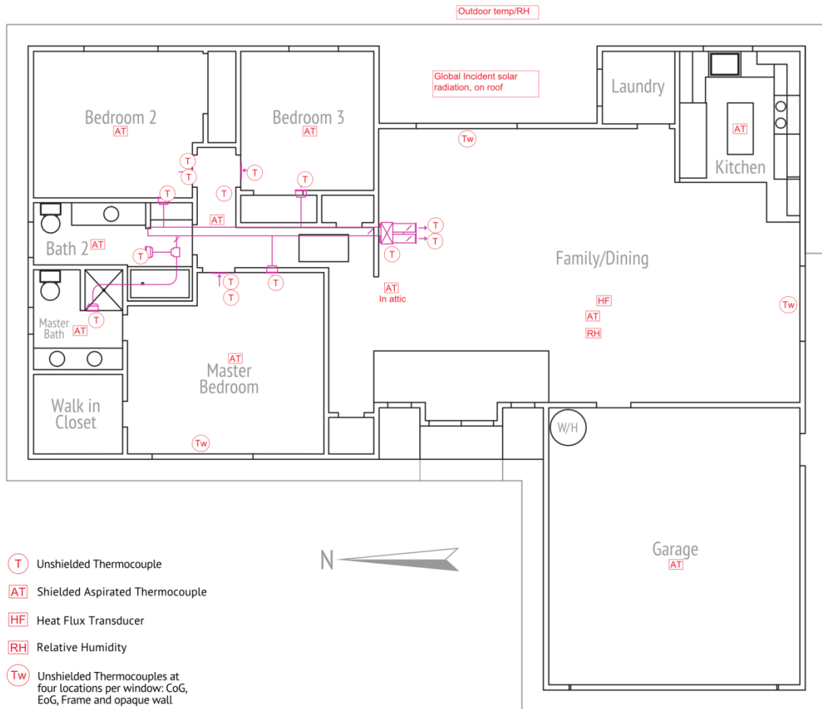
Figure 12. Sensor locations
