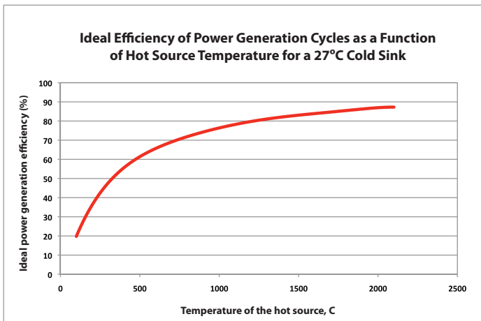
This chart illustrates the ideal efficiency of power generation cycles as a function of the temperature at which heat is transferred. The higher the temperature of heat transfer, the higher the cycle efficiency, and thus, the need for heat transfer fluids (HTFs) operating between 650° and 1200°C. Graphic from Argonne
