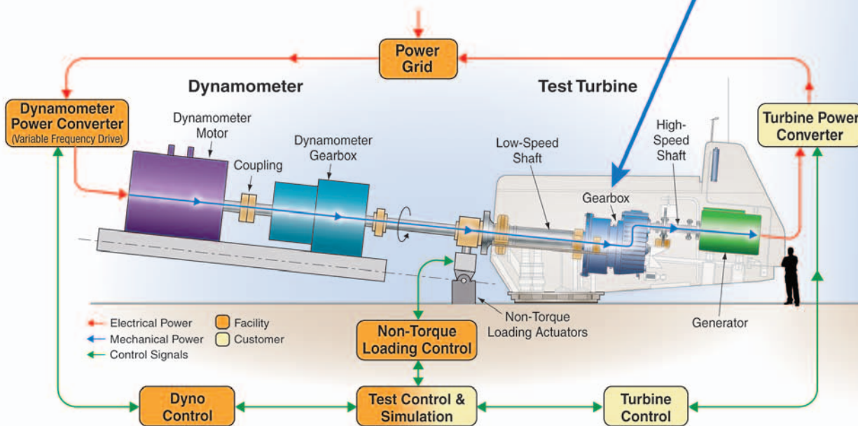
Dynamometer test configuration for a wind turbine drivetrain.
