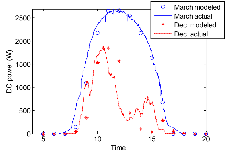
Modeled results (dots) and measured data (lines) for two representative sunny dates
