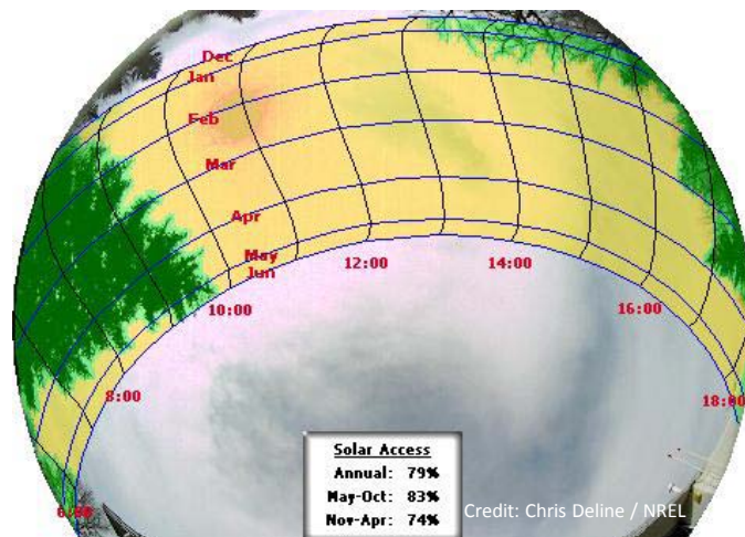
Site survey: ~20% irradiance loss due to shade
