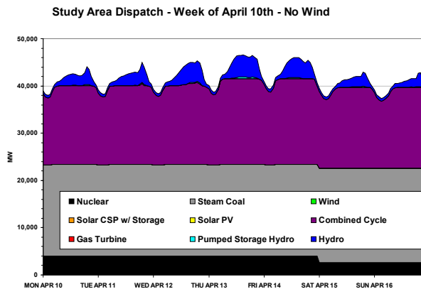
Fig. 2. Example of dispatch from April; no wind.
